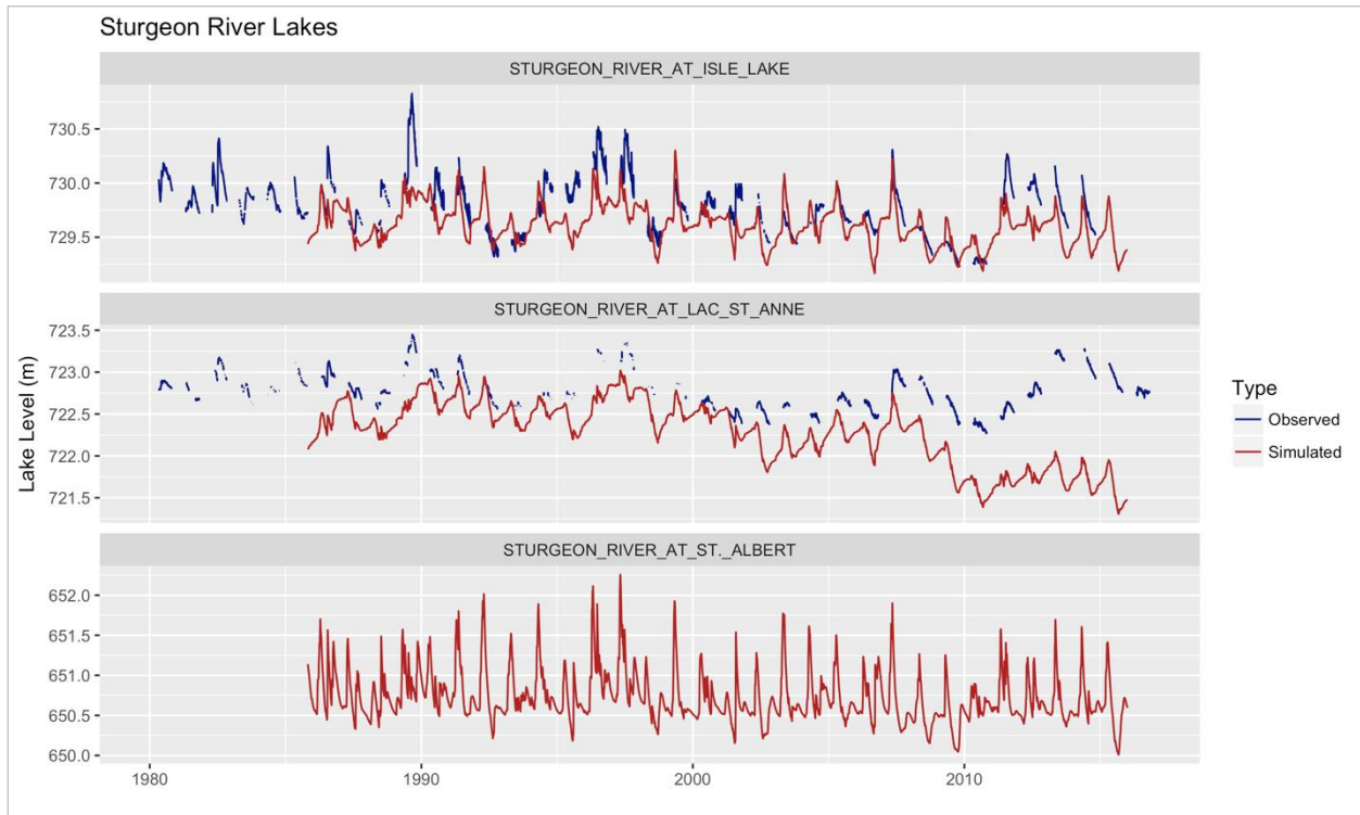
Figure 12. Simulated and observed water levels in three lakes modelled
