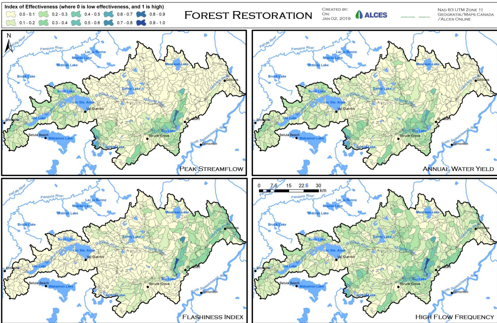
Figure 15. Response of peak streamflow, annual water yield, flashiness index, and high flow frequency to the forest restoration strategy.
