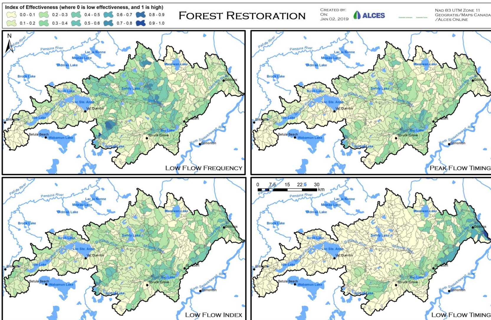
Figure 16. Response of flow flow frequency, peak flow timing, low flow index, and low flow timing to the forest restoration strategy.
