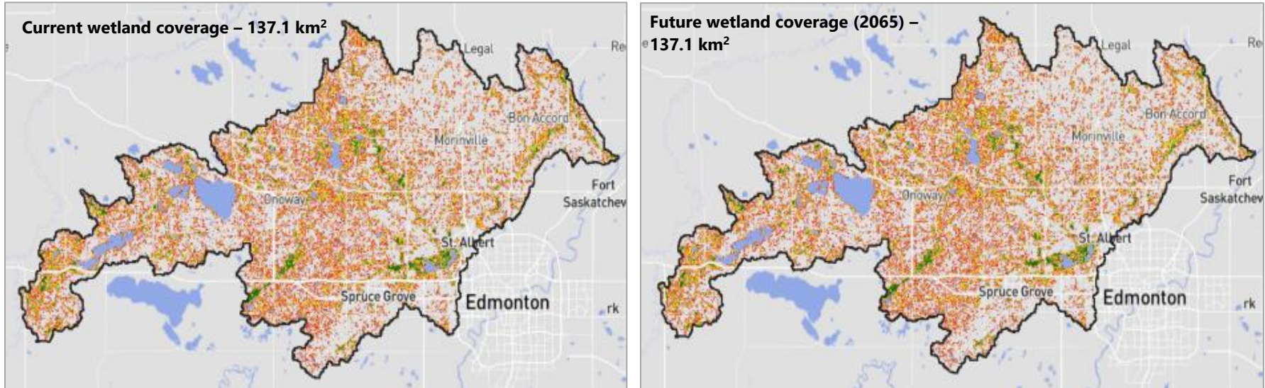
Figure 8. Current and future wetland coverage simulated using the wetland protection strategy.
