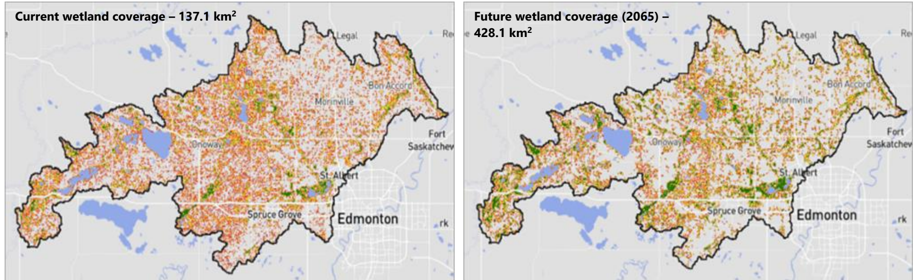
Figure 9. Current and future wetland coverage simulated using the wetland restoration strategy.
