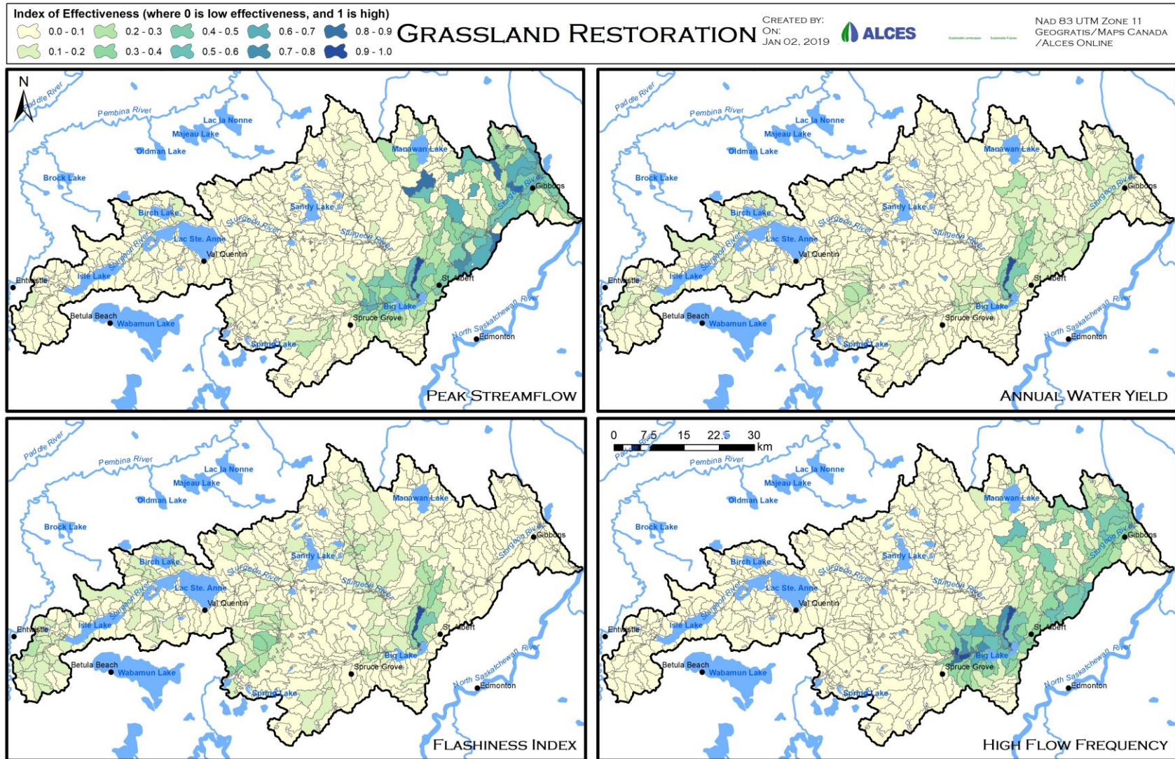
Figure 17. Response of peak streamflow, annual water yield, flashiness index, and high flow frequency to the grassland restoration strategy.
