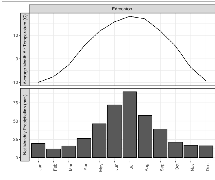
Figure 2. Average monthly air temperature and net monthly precipitation for the Edmonton climate station over the period from 1980-2016
