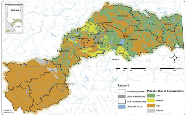
Map 23. Potential Risk of Groundwater Contamination based on Geological Setting
